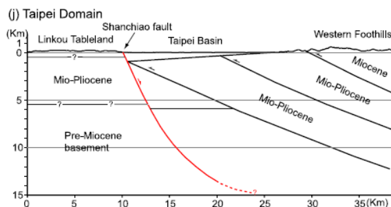
Fig. 2 Simple cross sections proposed for Taipei domains. Each crude, unbalanced cross section provides tentative geometries of the major active faults based upon geomorphic, geodetic, structural, and seismic data. Red indicates active structures;
