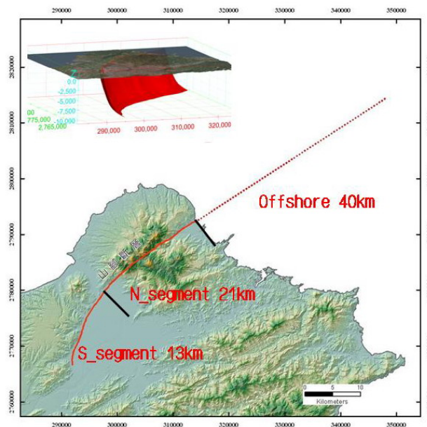
Fig. 1 The inland and offshore distribution of Shanchiao fault and the geometry of Shanchiao fault is shown at the upper left.
