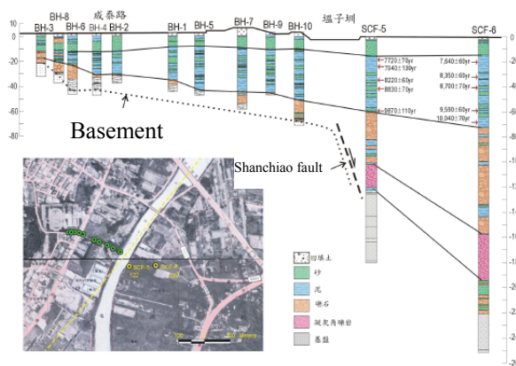
Fig. 3 The Chengtzuliao stratigraphic profile of boreholes in Taipei basin. (Liu et al., 2000; Su et al., 2003)
