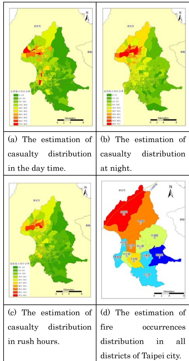
Fig. 8. We assumed that Shanchiao fault (dip angle 60E) ruptures 80km and occurs M_w 7.3 earthquake, and then considered the hanging wall effect and adopted the latest ground motion attenuation formula to estimate the earthquake loss in all districts of Taipei.
