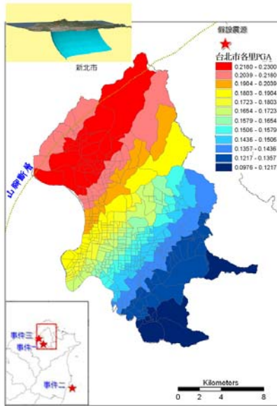
Fig. 7. The PGA distribution map of the three possible earthquake sources in 475 year return period (Peak Ground Acceleration PGA=0.23g ) in Taipei city. (a) Subduction zone interface at Ilan and Hualien offshore, (b) Subduction zone intraslab beneath Taipei Basin and (c) Shanchiao fault at Taipei basin.
