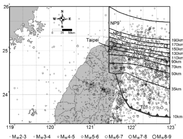
Fig. 4. Isobaths contours of the top of subducting Philippine Sea plate and spatial distribution of independent intermediate-depth and deep earthquakes (depth F 35 km) in northern Taiwan.
