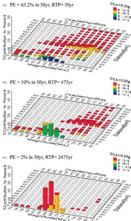
Fig. 6. Deaggregation of the total seismic hazard of Taipei in different Probability of exceedance (PE) and return period (RTP). (a) 50 yr return period; (b) 475 yr return period; (c) 2475 yr return period. The total seismic hazard is discrete in magnitude bins, distance bins and epsilon ( \epsilon ). The meaning of \epsilon is the expected PGA level scaled to number of standard deviation of ground motion relationship.
