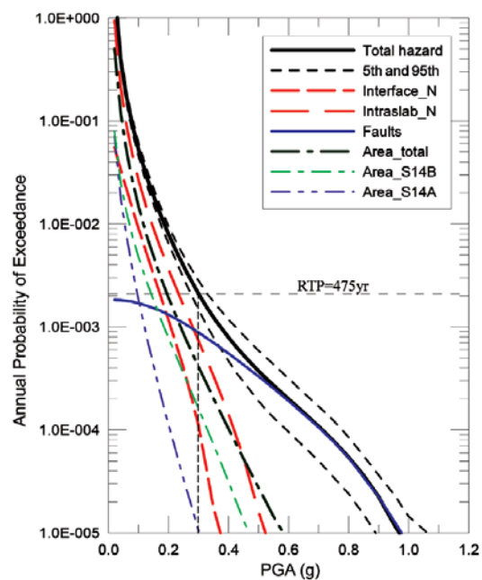
Fig. 5. Seismic hazard curves of PGA for Taipei city in soil site condition. The hazard curves of PGA present the total hazard in 5th, 50th (median), and 95th percentiles uncertainty in PSHA. In addition, the hazard contribution from the sources around Taipei to total hazard(s) is also shown in the figure in different line styles. The horizontal dashed line indicates the annual probability of exceedance in 1/475 representing 475-year return period, and the horizontal dashed line crosses over the total hazard curve at PGA 0.3 g is referred by a vertical dashed line.
